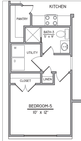
OPT. BEDROOM/BATH-3
